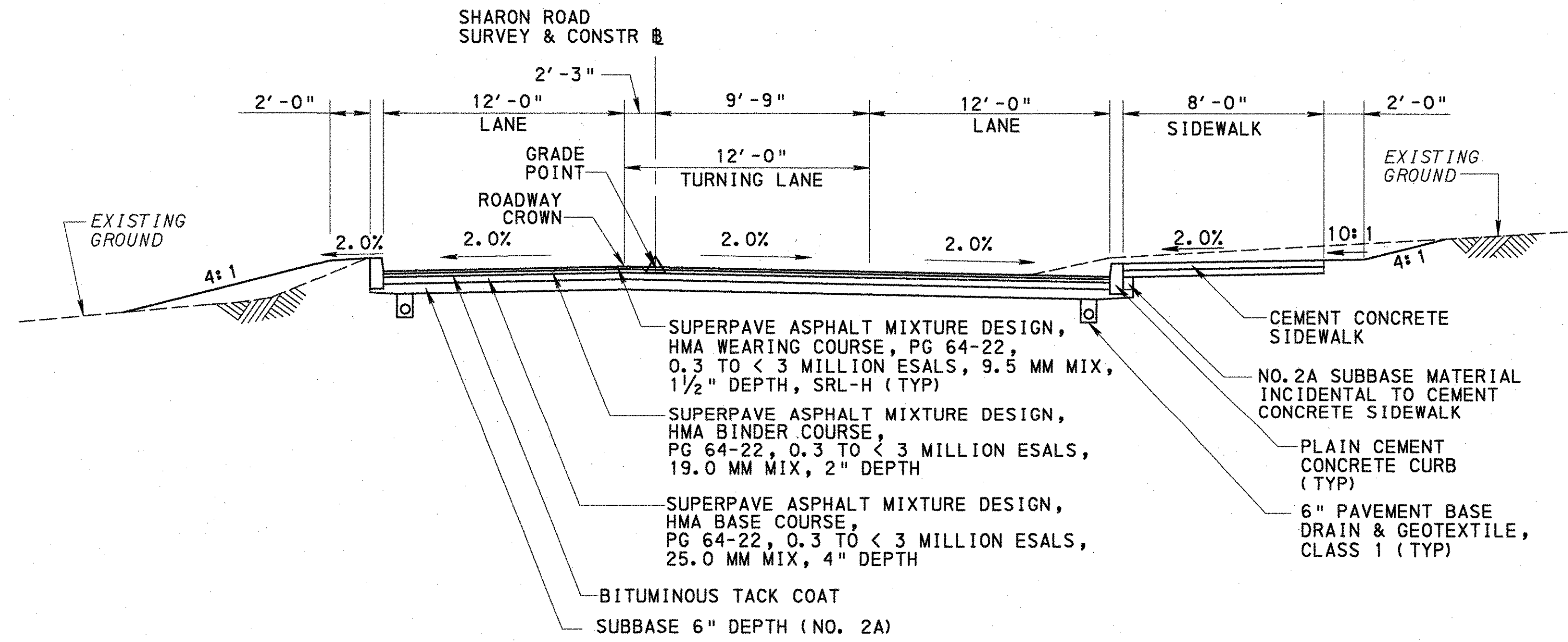
TYPICAL SECTION SHARON ROAD STA 5+42.69 TO STA 8+56.39 NOT TO SCALE
